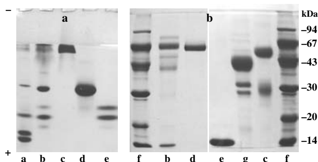
Fig. 2. Electrophoretic analysis of the purified camel whey protein using native PAGE (a) or SDS-PAGE (b). a: bovine whey; b: camel whey; c: purified IgG; d: purified albumin; e: purified \alpha -lactalbumin; f: molecular weight markers (phosphorylase b 94 kDa, bovine albumin 67 kDa, ovalbumin 43 kDa, carbonic anhydrase 30 kDa, trypsin inhibitor g 20.1 kDa, \alpha -lactalbumin 14.4 kDa); g: IgG 80 kDa (ascending part of the third peak obtained by chromatography of camel serum on Sephadex G200).
